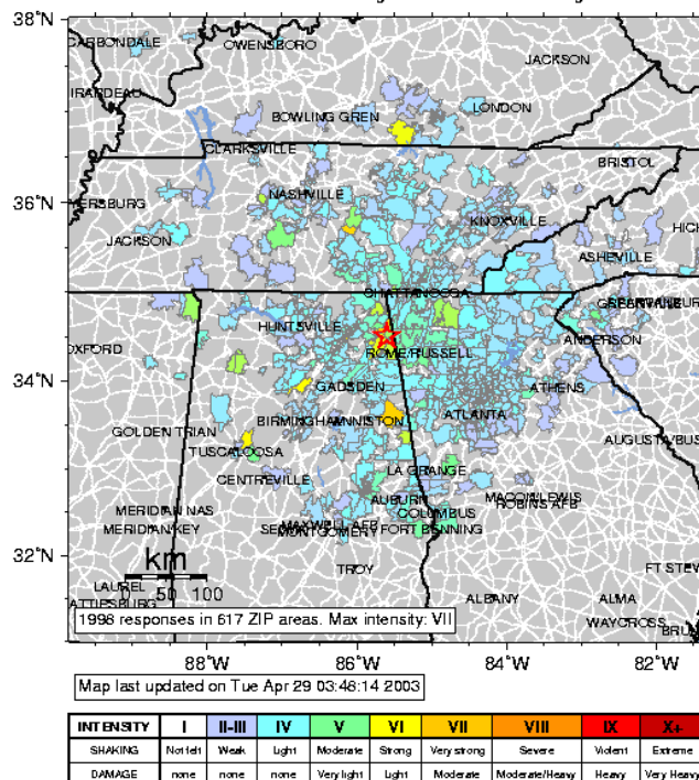
Community Internet Intensity Map (8 miles ENE of Fort Payne, Alabama) ID:teak 03:59:37 CDT APR 29 2003 Mag=4.9 Latitude=N34.51 Longitude=W85.60
